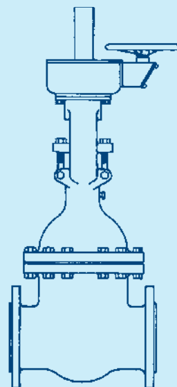
BEVEL GEARING WITH HORIZONTAL HANDWHEEL
