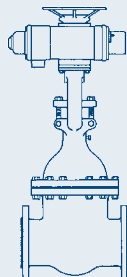
ELECTRIC ACTUATOR
